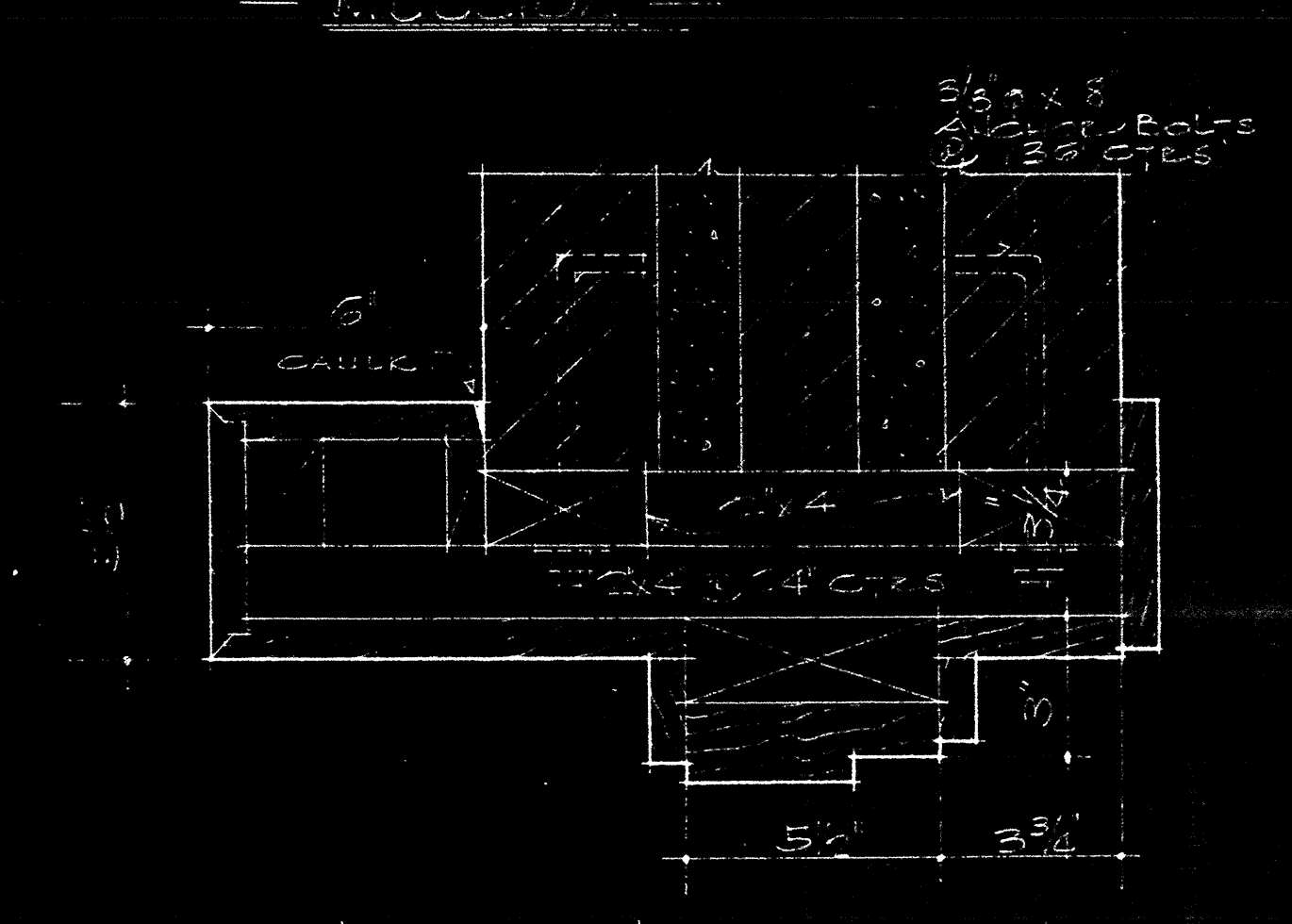
DETAILS AT WINDOW "B" - DOOR "116" SIMILAR AT WINDOWS "D" & "C" - DOOR "108" SCALE 3/4" = 1'-0"
