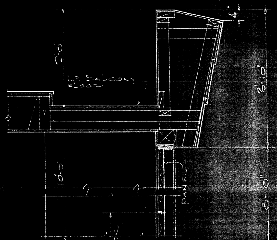
DETAIL - WINDOW "B" SCALE 3/4" = 1'-0"
